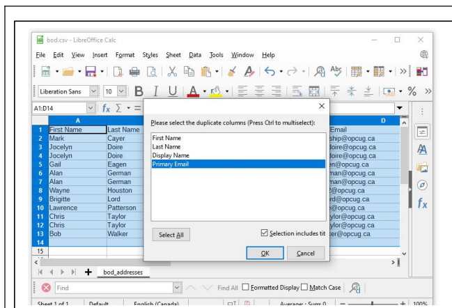
Figure 1. Original dataset
